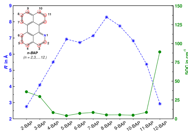
Fig. 4 Distance between Br and N ( R in Å) in n -BAP and the SOC between the ^1\pi\pi^* and ^3\text{n}\pi^* states ( \langle ^1\pi\pi^* | \hat{H}_{\text{so}} | ^3\text{n}\pi^* \rangle in \text{cm}^{-1} ).
