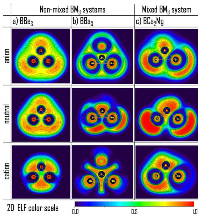
Fig. 4 Cut-plane electron localization function (ELF) plots of representative (a) and (b) non-mixed and (c) mixed anionic (top), neutral (middle), and cationic (bottom) \text{BAe}_3 clusters in the B–Ae 1 –Ae 2 plane. The ELF plots were obtained with the Multiwfn v.3.8. software. 42,43
