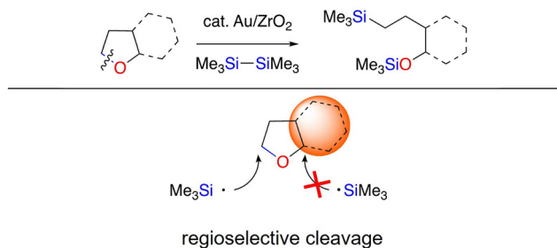
Fig. 1 Reaction scheme of Au/ZrO 2 -catalyzed silylation of ethers with C(sp 3 )-O bonds using disilanes to produce alkylsilanes.
