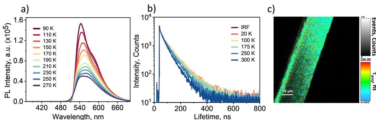
Fig. 3 (a) Steady-state photoluminescence spectra and (b) lifetime decay plots at indicated temperatures and (c) FLIM of the PYDB–TCNB cocrystal.
