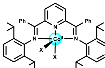
X = Cl; Sq. Pyramidal, d = 0.57 \text{ \AA} , D = -72 \text{ cm}^{-1} . X = Br; Sq. Pyramidal, d = 0.54 \text{ \AA} , D = -67 \text{ cm}^{-1} . X = I; Sq. Pyramidal, d = 0.46 \text{ \AA} , D = -25 \text{ cm}^{-1} .
