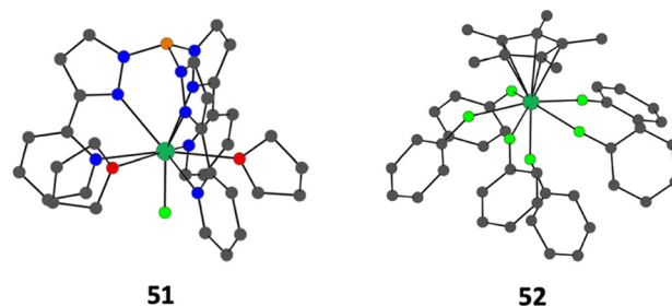
Fig. 7 Solid-state structures of the cations from [Dy(Tp^{2-py})F(THF)_2]PF_6 ( 51 ) and [Dy(Cp^*)(\kappa^1-FC_6H_5)_6][Al(OC(CF_3)_3)_3]_2(\mu-F)_2 ( 52 ). Dysprosium(III) = turquoise, fluorine = fluoro-green, oxygen = red, nitrogen = blue, carbon = grey, and boron = orange; hydrogen atoms have been omitted clarity. 73,74
