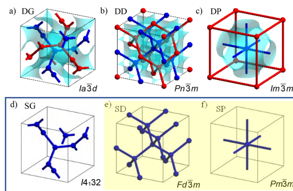
Fig. 1 (a)–(c) Double network cubic phases with corresponding space groups and their infinite minimal surfaces (blue) and (d)–(f) the corresponding single networks. Reproduced from ref. 16.
