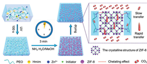
Fig. 13 Schematic illustration of the ZIF/PEO membrane preparation. Adapted from ref. 70 with permission from the John Wiley and Sons.
