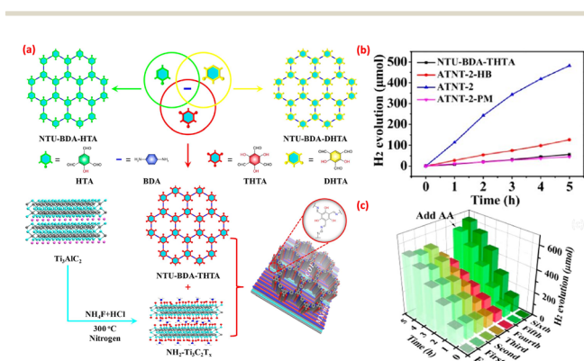
Fig. 12 (a) Synthesis of the COF/MXene-NH 2 hybrid; (b) photocatalytic activity of synthesized hybrids; and (c) recyclability. Reprinted with permission from ref. 35. Copyright 2020 American Chemical Society.
