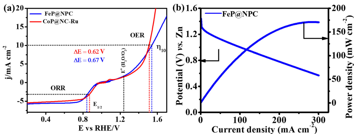
Fig. 9 (a) Polarization curves of FeP@NPC and CoP@NC-Ru demonstrating their bifunctional oxygen activity. (b) Discharge polarization curve of FeP@NPC showing the power density. Adapted from ref. 63 and 105.
