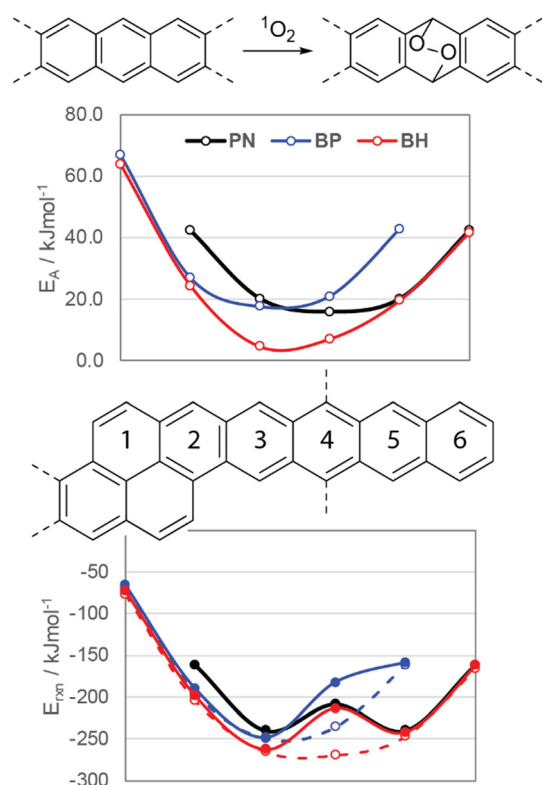
Fig. 6 (top) Activation energies and (bottom) reaction energies of bisacenes with singlet oxygen at different ring positions. Open circles are without the silylethynyl groups, and filled circles are with these groups included. All energies computed with M06-2X/cc-pVTZ.
