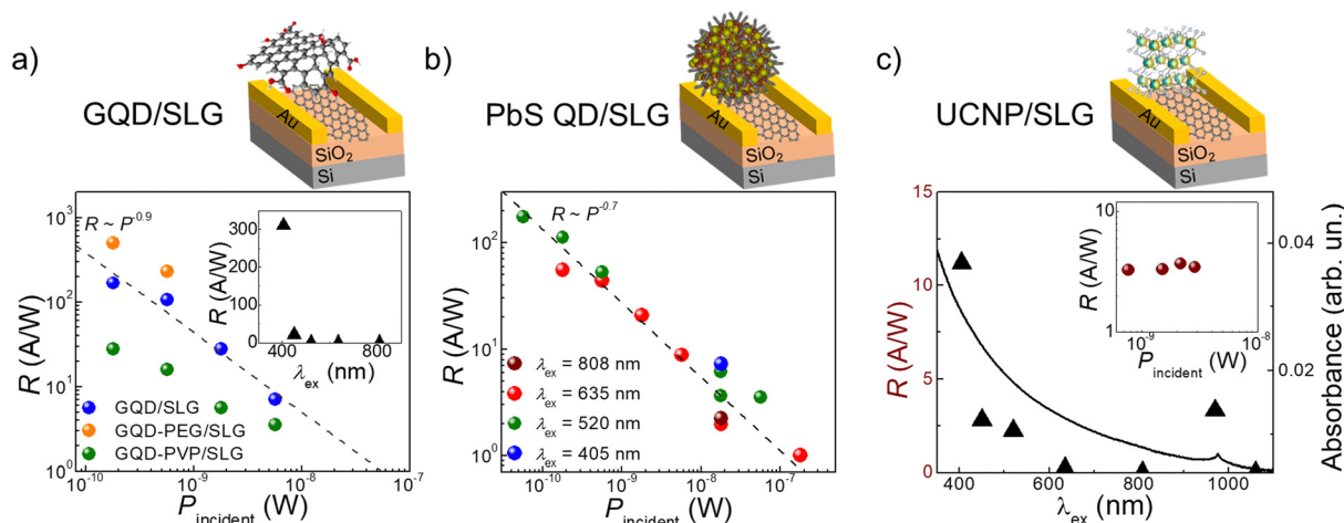
Fig. 3 (a) Photoresponsivity, R , as a function of incident light power on the sample, P_{\text{sample}} , for the GQD/SLG, GQD-PEG/SLG and GQD-PVP/SLG devices. ( V_{\text{sd}} = 2 \text{ mV} , V_{\text{g}} = 0 \text{ V} , \lambda_{\text{ex}} = 405 \text{ nm} ). Inset: R as a function of excitation wavelength, \lambda_{\text{ex}} , for the GQD/SLG ( V_{\text{sd}} = 2 \text{ mV} , V_{\text{g}} = 0 \text{ V} , P = 179 \text{ W m}^{-2} ) device. (b) R as a function of P_{\text{sample}} for printed PbS QD/SLG device ( V_{\text{sd}} = 4 \text{ mV} , V_{\text{g}} = 0 \text{ V} ) for different \lambda_{\text{ex}} values ( V_{\text{sd}} = 4 \text{ mV} , V_{\text{g}} = 0 \text{ V} ). (c) R as a function of \lambda_{\text{ex}} for printed UCNP/SLG device ( V_{\text{sd}} = 2 \text{ mV} , V_{\text{g}} = 0 \text{ V} , P = 5.7 \text{ W m}^{-2} ), with absorption spectra of UCNPs shown for comparison. Inset: R as a function of P_{\text{sample}} for printed UCNP/SLG device ( V_{\text{sd}} = 2 \text{ mV} , V_{\text{g}} = 0 \text{ V} , \lambda_{\text{ex}} = 970 \text{ nm} ).
