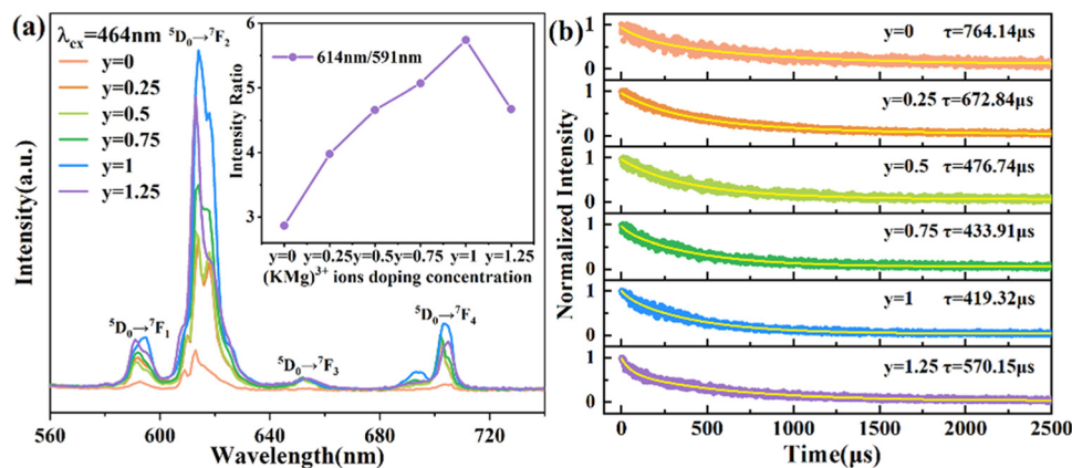
Fig. 4 (a) Photoluminescence emission spectra of (\text{KMg})_y\text{Sc}_{2-y}\text{W}_3\text{O}_{12}:1 \text{ mol}\% \text{Eu}^{3+} ( y = 0, 0.25, 0.5, 0.75, 1, \text{ and } 1.25 ) phosphors, inset: the intensity ratio \beta with different (\text{KMg})^{3+} concentrations. (b) Photoluminescence decay curves of \text{Eu}^{3+}: ^5\text{D}_0 .
