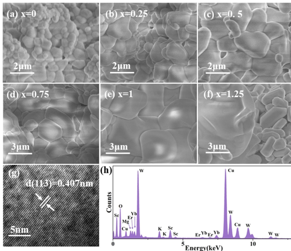
Fig. 3 (a)–(f) SEM images of (\text{KMg})_y\text{Sc}_{2-y}\text{W}_3\text{O}_{12}:1 \text{ mol}\% \text{Er}^{3+}/20 \text{ mol}\% \text{Yb}^{3+} ( x = 0, 0.25, 0.5, 0.75, 1, \text{ and } 1.25 ) phosphors. (g) HRTEM image and (h) EDX results of the (\text{KMg})\text{ScW}_3\text{O}_{12}:1 \text{ mol}\% \text{Er}^{3+}/20 \text{ mol}\% \text{Yb}^{3+} phosphor.
