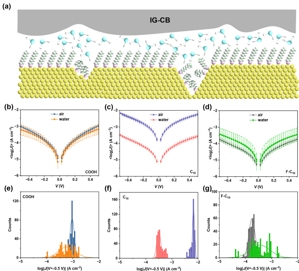
Fig. 2 (a) The scheme of molecular junctions conducted in water. (b) Plots of the \langle \log|J(V)| \rangle curves for Au TS -SC 9 COOH//IG-CB junctions tested in air and water. (c) Plots of the \langle \log|J(V)| \rangle curves for Au TS -SC 10 //IG-CB junctions tested in air and water. (d) Plots of the \langle \log|J(V)| \rangle curves for Au TS -SC 10 F//IG-CB junctions tested in air and water. (e)–(g) The corresponding histograms of \log|J| at -0.5 V with Gaussian fits.
