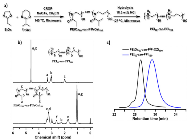
Fig. 1 Overview copolymer synthesis and analysis. Panel (a): synthesis scheme for the preparation of L-PEI 60 -ran-PPI 190 copolymer. Panel (b): 1 H NMR spectra of PEIOx 60 -ran-PPI 190 and L-PEI 60 -ran-PPI 190 in CDCl 3 and D 2 O, respectively. Panel (c): SEC traces of PEIOx 60 -ran-PPI 190 in DMA and L-PEI 60 -ran-PPI 190 in aqueous medium.
