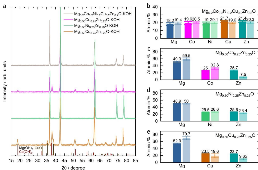
Fig. 7. (a) XRD patterns of \text{Mg}_{0.2}\text{Co}_{0.2}\text{Ni}_{0.2}\text{Cu}_{0.2}\text{Zn}_{0.2}\text{O} and \text{Mg}_{0.50}\text{TM}_{0.25}\text{Zn}_{0.25}\text{O} (TM = Co, Ni, Cu) after soaking in 2 M KOH for four weeks, denoted as \text{Mg}_{0.2}\text{Co}_{0.2}\text{Ni}_{0.2}\text{Cu}_{0.2}\text{Zn}_{0.2}\text{O-KOH} and \text{Mg}_{0.50}\text{TM}_{0.25}\text{Zn}_{0.25}\text{O-KOH} . XRD standard peak: \text{Mg}(\text{OH})_2 refers to PDF 00-007-0239; \text{Co}(\text{OH})_2 refers to PDF 00-045-0031; \text{CuO} refers to PDF 00-045-0937. Atomic percentage of
