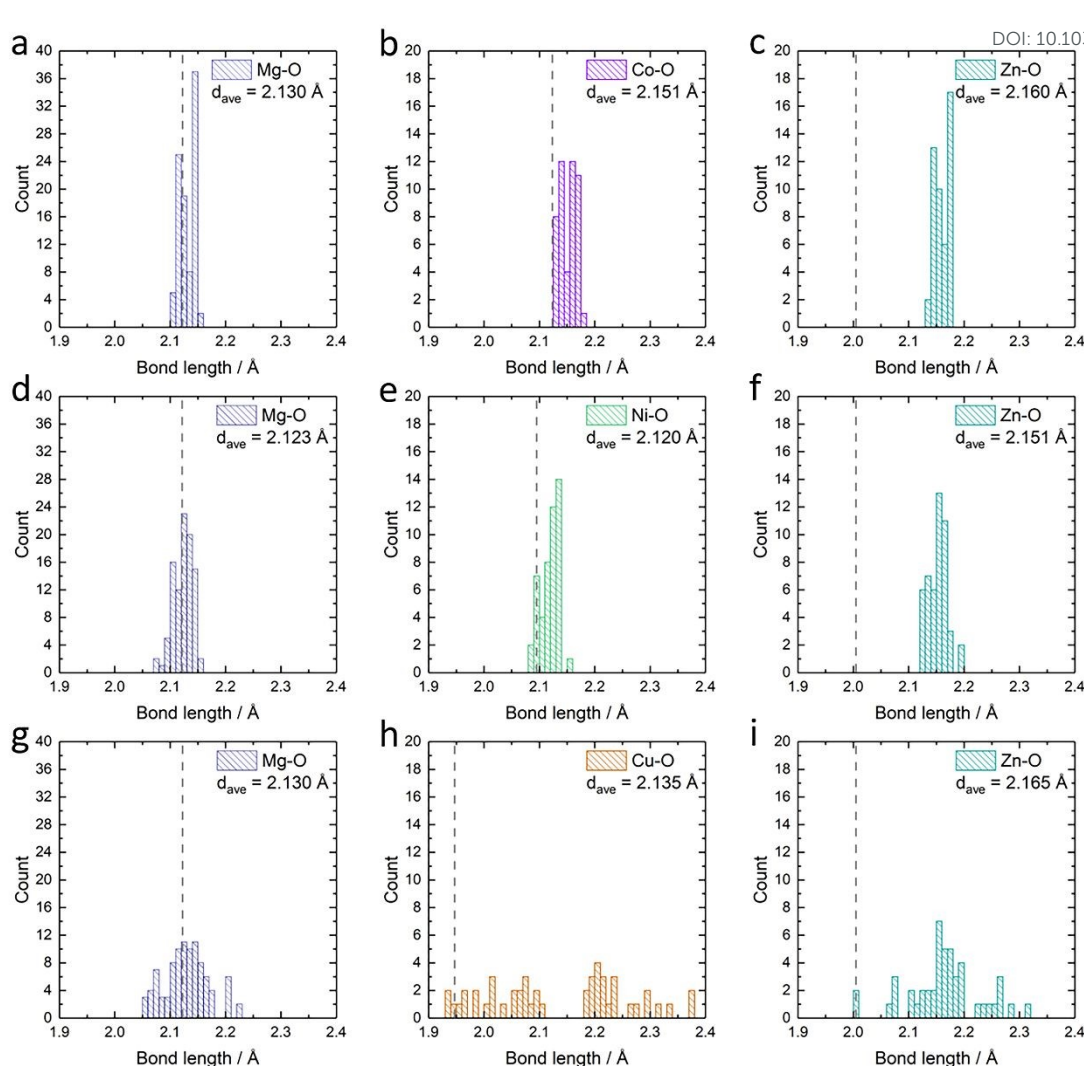
Fig. 6. The statistics of the metal-oxygen bond length in the relaxed structure: the bond-length of (a) Mg-O, (b) Co-O and (c) Zn-O in \text{Mg}_{0.50}\text{Co}_{0.25}\text{Zn}_{0.25}\text{O} ; the bond-length of (d) Mg-O, (e) Ni-O and (f) Zn-O in \text{Mg}_{0.50}\text{Ni}_{0.25}\text{Zn}_{0.25}\text{O} ; the bond-length of (g) Mg-O, (h) Cu-O and (i) Zn-O in \text{Mg}_{0.50}\text{Cu}_{0.25}\text{Zn}_{0.25}\text{O} . d_{\text{ave}} stands for the average metal-oxygen bond length in each panel. The dash lines indicate the calculated metal-oxygen bond length for metal monoxides: rock-salt MgO in (a), (d) and (g), rock-salt CoO in (b); rock-salt NiO in (e), tenorite CuO in (h), wurtzite ZnO in (c), (f) and (i).
