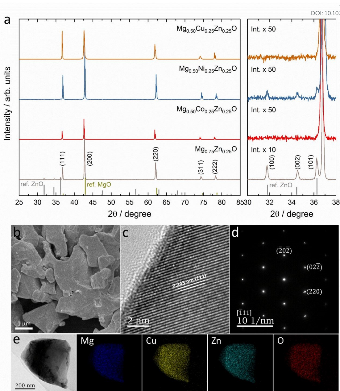
Fig. 1. (a) XRD patterns of Co, Ni and Cu substituted \text{Mg}_{0.75}\text{Zn}_{0.25}\text{O} . XRD standard peak: MgO refers to PDF 00-045-0946 and ZnO refers to PDF 00-036-1451. (b) SEM image, (c) HRTEM image, (d) SAED pattern at the location in (c), and (e) TEM-mapping of \text{Mg}_{0.50}\text{Cu}_{0.25}\text{Zn}_{0.25}\text{O} .
