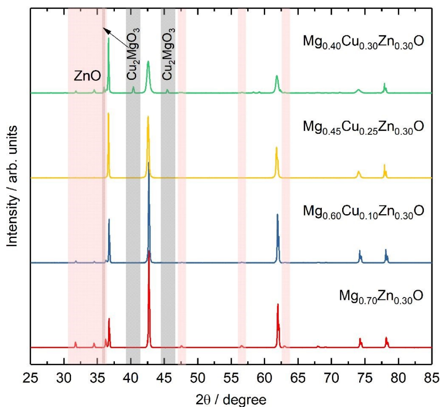
Fig. 4. XRD patterns of \text{Mg}_{0.70-x}\text{Cu}_x\text{Zn}_{0.30}\text{O} series.
