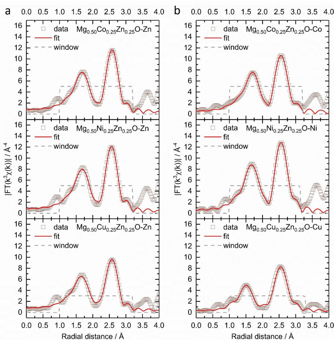
Fig. 2. The k^3 -weighting FT-EXAFS and the fitting of (a) Zn K-edge and (b) Co, Ni and Cu K-edges of \text{Mg}_{0.50}\text{TM}_{0.25}\text{Zn}_{0.25}\text{O} (TM = Co, Ni, Cu) under a Hanning-shaped window.
