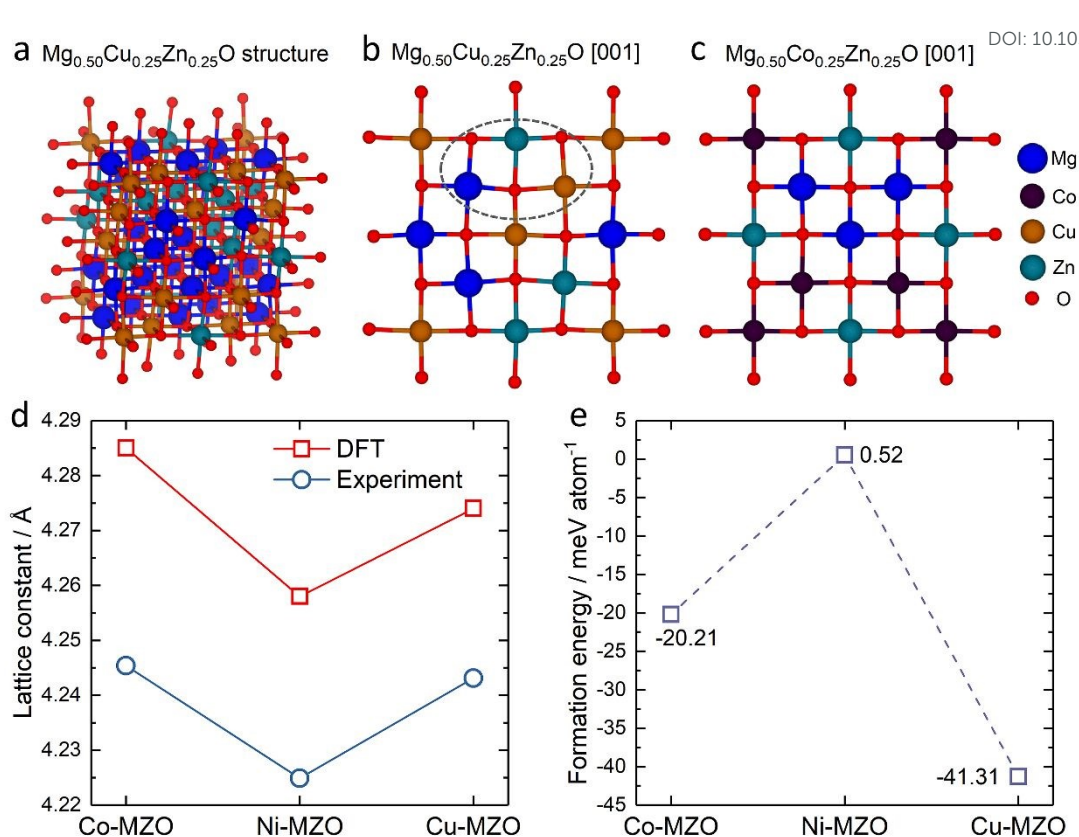
Fig. 5. The typical rock-salt structure generated from the high-entropy random model of (a) \text{Mg}_{0.50}\text{Cu}_{0.25}\text{Zn}_{0.25}\text{O} , the slice of (b) \text{Mg}_{0.50}\text{Cu}_{0.25}\text{Zn}_{0.25}\text{O} and (c) \text{Mg}_{0.50}\text{Co}_{0.25}\text{Zn}_{0.25}\text{O} viewed from [001] direction; (d) the lattice constant from the relaxed structure and the experiment (XRD patterns), and (e) the average formation energy for substituting Mg by Zn in \text{Mg}_{0.50}\text{Co}_{0.25}\text{Zn}_{0.25}\text{O} (Co-MZO), \text{Mg}_{0.50}\text{Ni}_{0.25}\text{Zn}_{0.25}\text{O} (Ni-MZO) and \text{Mg}_{0.50}\text{Cu}_{0.25}\text{Zn}_{0.25}\text{O} (Cu-MZO).
