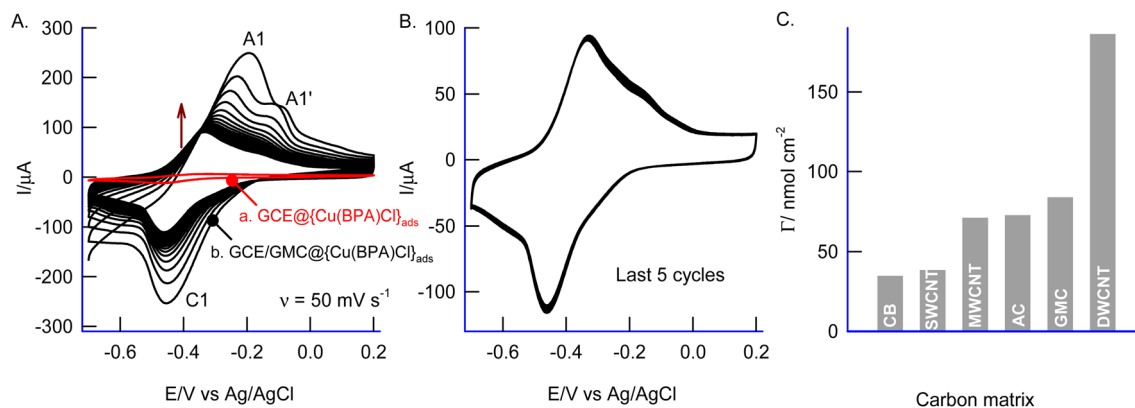
Fig. 1 (A) Cyclic voltammetric responses of (a) \text{GCE}@{\text{Cu}(\text{BPA})\text{Cl}}_{\text{ads}} ; (b) \text{GCE}/\text{GMC}@{\text{Cu}(\text{BPA})\text{Cl}}_{\text{ads}} in nitrogen purged 0.1 M PBS, pH 7, at scan rate ( \nu ) = 50 \text{mV s}^{-1} ( n = 20 cycles) and (B) last five CVs; (C) comparative plots of surface excess values of different carbon nanomaterials used.
