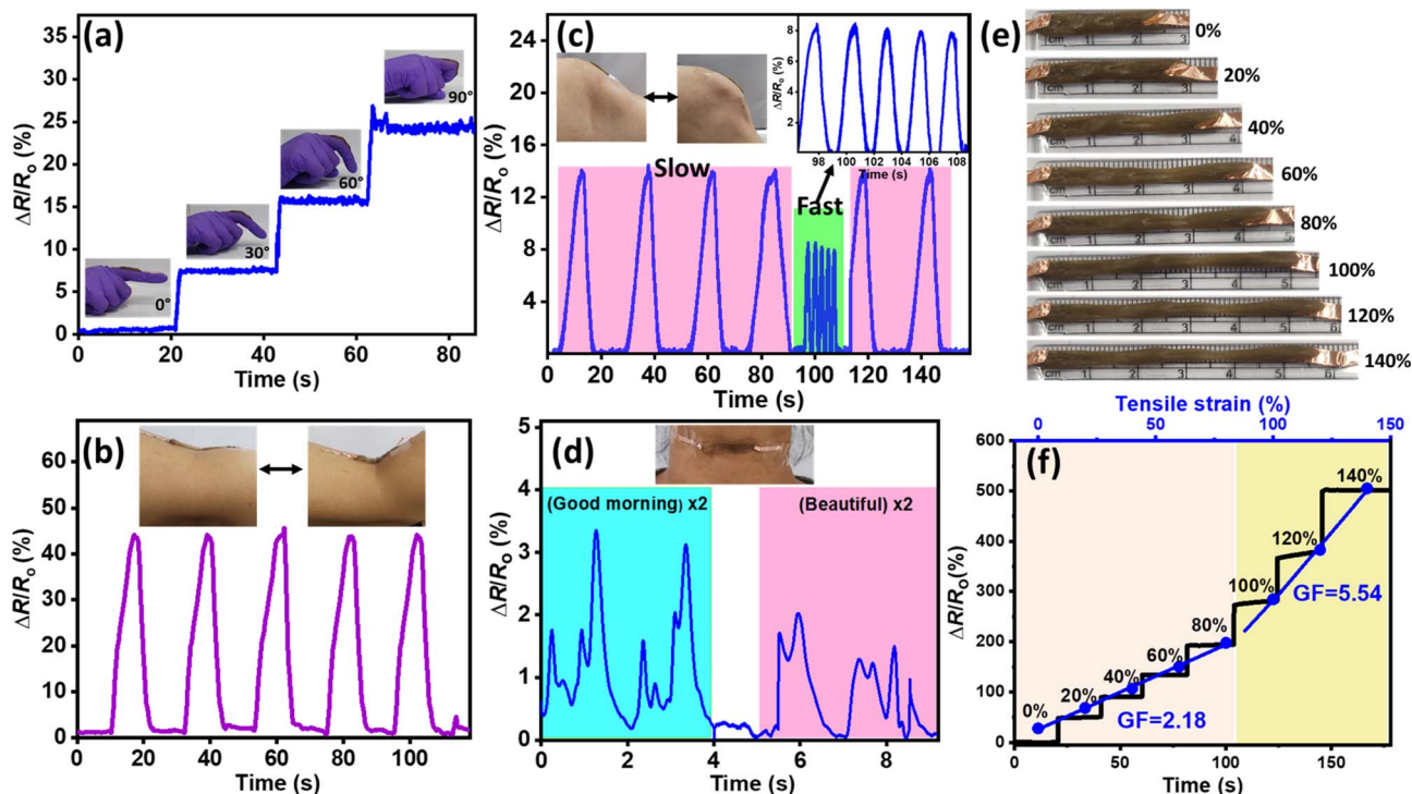
Fig. 7 Real-time monitoring of the PVIM-PPA-Ca (3c) ion-gel-based wearable strain sensor for various human activities. Signals of the relative resistance change ( \Delta R/R_0 ) of 3c as a function of (a) finger bending at various angles, (b) arm bending, (c) knee bending, and (d) speaking different words; (e) photograph of 3c at various applied strains; (f) corresponding relative resistance ( \Delta R/R_0 ) and gauge factors.
