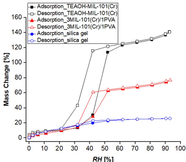
Fig. 11 Water adsorption–desorption isotherms ( T = 25\text{ }^{\circ}\text{C} ) of TEOAH-MIL-101(Cr), 3MIL-101(Cr)/1PVA and the silica gel control.
