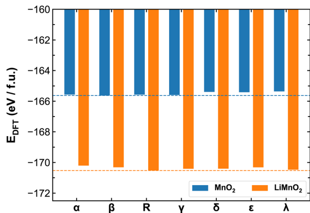
Fig. 3 Ab initio energies of different \text{MnO}_2 and \text{LiMnO}_2 polymorphs calculated using the SCAN functional. The dash lines mark the lowest energies obtained for \beta - \text{MnO}_2 and R- \text{LiMnO}_2 .
