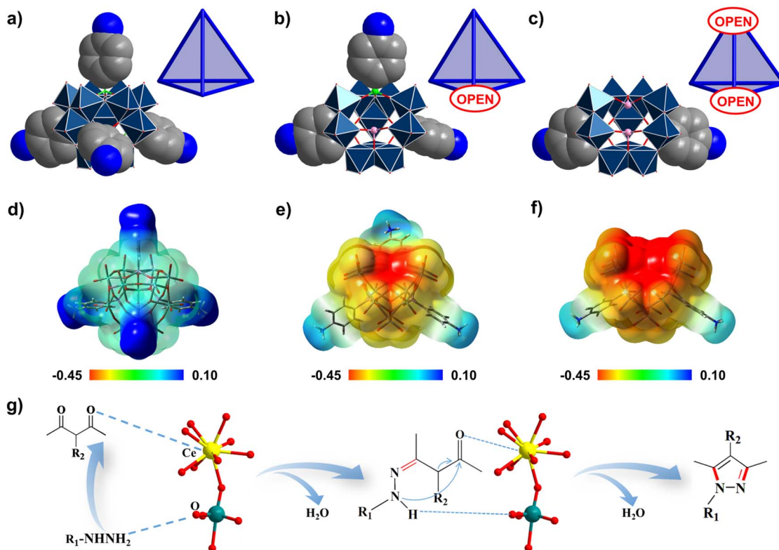
Fig. 5 (a)–(c) Transition of the Mo–oxo frameworks from fully closed ( \text{As}_4\text{Mo}_{12} ) to gradually open structures ( \text{SeAs}_3\text{Mo}_{10} (b); \text{Se}_2\text{As}_2\text{Mo}_{10} (c)). (d)–(e) Molecular electrostatic potential (MEP) distribution (isovalue 0.02) for \text{As}_4\text{Mo}_{12} (d), \text{SeAs}_3\text{Mo}_{10} (e), and \text{Se}_2\text{As}_2\text{Mo}_{10} (f). The red areas are more nucleophilic regions. (g) Proposed catalytic synergistic effect of the \text{Ce}^{\text{III}} ions in \text{Se}_2\text{As}_6\text{Mo}_{20}\text{Ce}_2 . Color code: Ce, yellow; Mo, cyan; O, red.
