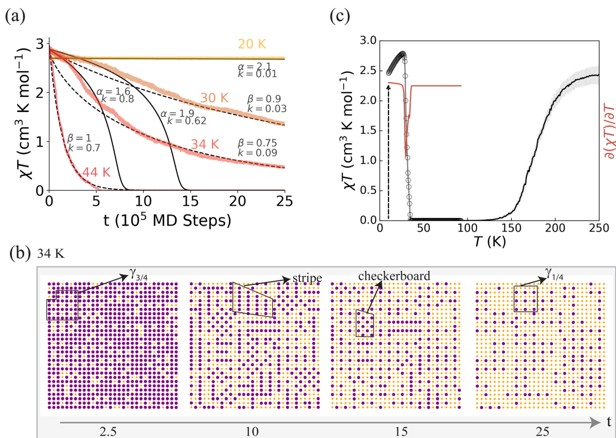
Fig. 6 Complex isothermal relaxation from a rugged free energy landscape and dynamical disorder due to competing phases in a model with a single SCO species. (a) Isothermal relaxation as it proceeds. At short times and low temperatures the relaxation is sigmoidal (eqn (1); solid line; parameters as marked); at long times and high temperatures the relaxation follows a stretched exponential form ( e^{-\kappa t^\beta} , \beta < 1 ; dashed line; parameters as marked). (b) The spin-state evolution at 34 K shows microdomains domains of competing chequerboard, stripe, \gamma_{1/4} and \gamma_{3/4} phases. (c) For these parameters, thermal SCO and thermally activated relaxation are both single-step processes. Here \kappa_3 = -0.15\kappa_1 , with the rest of the parameters as listed in Tables 1 and S1.†
