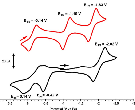
Fig. 3 Cyclic voltammograms of 1 (bottom, black) and 2 (top, red) in 0.1 M [ n -Bu 4 N][PF 6 ] solution (scan rate = 100 mV s -1 ). All potentials are referenced to Fc/Fc + .
