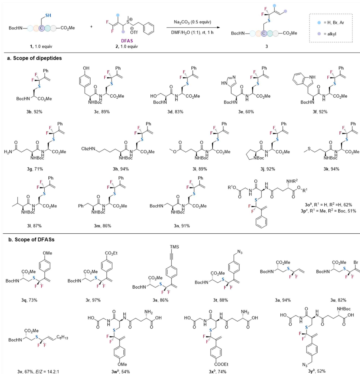
Scheme 1 S-gem -Difluoroallylation of cysteine-containing dipeptides and tripeptides with DFAS 2. a Reaction conditions: 1 (0.2 mmol, 1.0 equiv.), 2 (1.0 equiv.), \text{Na}_2\text{CO}_3 (0.5 equiv.), H 2 O (2 mL), DMF (2 mL), rt, 1 h. b 2.5 equiv. \text{Na}_2\text{CO}_3 was added. c The reaction was carried out on a 1 mmol scale. All reported yields are isolated yields.
