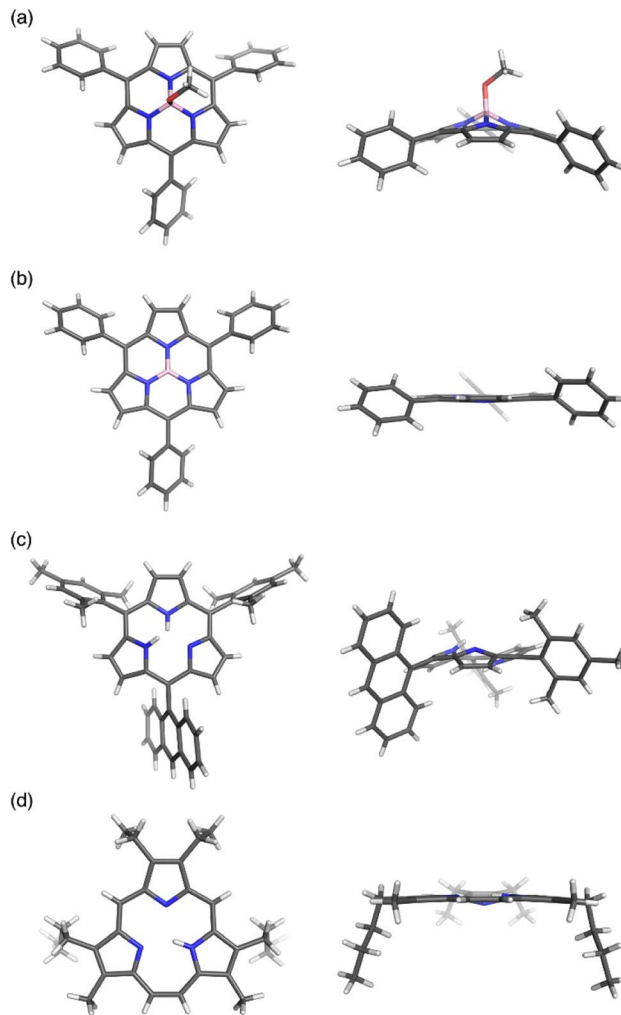
Fig. 2 X-ray crystal structures of (a) meso -phenyl subporphyrin 8 , (b) subporphyrin borenium cation 66 , (c) subporphyrin free-base 25 , and (d) tripyrryn(2.1.1) 38 . Left: top view, right: side view.
