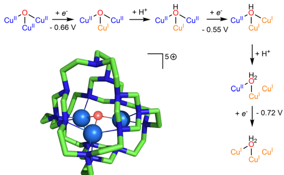
Fig. 11 Stepwise proton-coupled reduction of the [\text{Cu}_3^{\text{II}}(\mu\text{-O})_3(\text{LH})]^{5+} complex ( \text{L} = \text{tren}_4 ) studied by Zhang as a model of multicopper oxidases for the reduction of dioxygen into water. Adapted from ref. 238.
