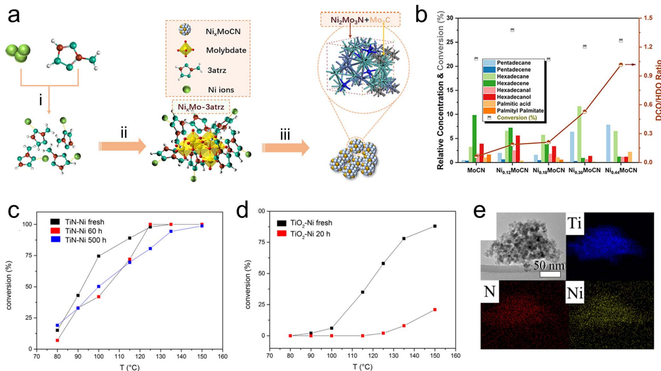
Fig. 6 TMNs for biomass upgrading. (a) Scheme showing synthesis procedure of Ni_xMoCN via (a) reaction of Ni nitrate and 3-amino-1,2,4-triazole (3atzr), (ii) addition of Mo to produce organic-inorganic precursor, and (iii) in situ pyrolysis. (b) Product distribution during the reaction of methyl palmitate. (c and d) Conversion of benzyl phenyl ether after continuous reaction of Kraft lignin for 20 h, 60 h, or 500 h. (e) XDS mapping of TiN-Ni catalyst. (a and b) Reprinted from ref. 100 with permission from the American Chemical Society, Copyright 2022. (c–e) Reprinted from ref. 106 with permission from the American Chemical Society, Copyright 2016.
