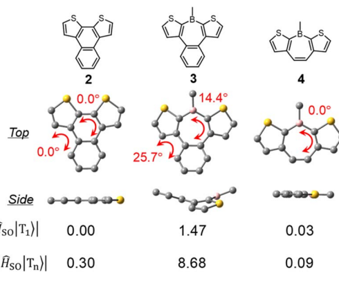
Fig. 8 DFT-optimized S 0 geometries of model compounds and their SOCMEs in cm -1 .
