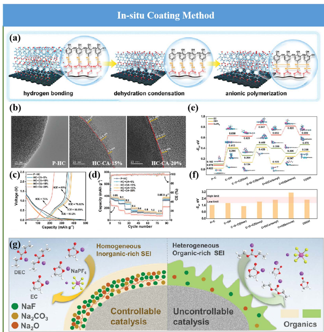
Fig. 12 (a) Illustration of the surface-functionality-reconstruction strategy of HC anodes, (b) TEM images of the HC anodes with different contents of CA, (c) GCD curves and (d) rate performances for HC anodes. (e) Binding energies of EC, DEC and NaPF 6 and (f) Na + adsorption energies by different oxygen-functional groups. (g) Diagram of SEI formation under a controllable catalysis mechanism in an ester electrolyte.
