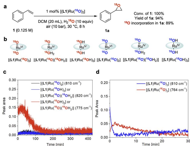
Fig. 7 ^{18}O isotope labelling experiments. (a) ^{18}O isotopic labelling experiment using ^{18}OH_2 . Conversion and yield determined by quantitative ^1H NMR spectroscopy, ^{18}O incorporation in 1a determined by GC-MS. (b) ^{18}O/^{16}O isotope labelled ruthenium species observed by FlowRaman spectroscopy. (c) Profile of Ru species observed by FlowRaman spectroscopy (reaction conditions as in Fig. 7a). (d) Profile of Ru species observed by in situ Raman spectroscopy (see Fig. S14 in the ESI†).
