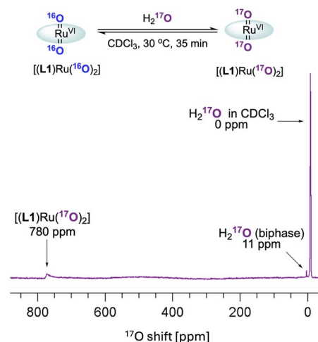
Fig. 8 ^{17}O NMR spectrum of [(L1)Ru^{VI}(^{16}O)_2] with ^{17}OH_2 in CDCl_3 .
