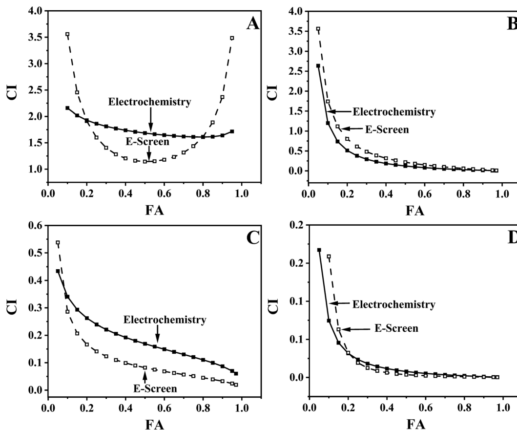
Fig. 6 FA-CI diagram evaluating the combined estrogenic effects of PGRs at actual environmental concentration ratios using electrochemical and E-Screen methods. (A) \text{GA}_3:\text{ETH} = 1:5 , (B) \text{GA}_3:\text{NAA} = 4:1 , (C) \text{ETH}:\text{NAA} = 20:1 , (D) \text{GA}_3:\text{ETH}:\text{NAA} = 4:20:1 .
