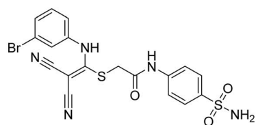
2-[1-(3-Bromophenylamino)-2,2-dicyanovinylthio]-N-(4-sulfamoylphenyl)acetamide
