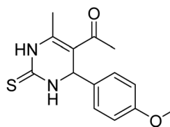
1-(4-(4-Methoxyphenyl)-6-methyl-2-thioxo-1,2,3,4-tetrahydropyrimidin-5-yl)ethanone
