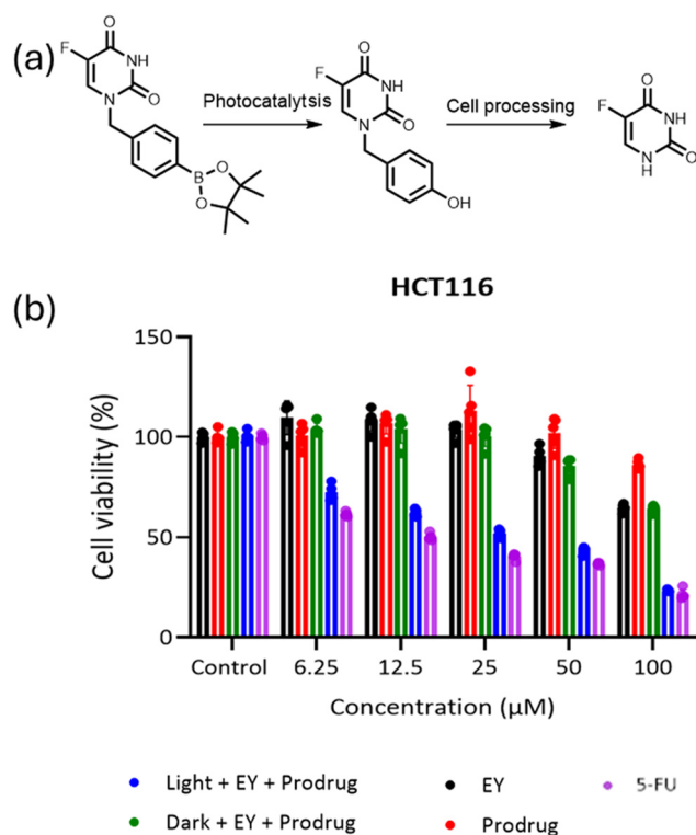
Fig. 5 The viability of HCT116 cancer cells treated with varying concentrations of the prodrug, PEG 113 - b -PAEMAH + 50 -EYHEMA 1 (shortened as EY), the combination of the prodrug and PEG 113 - b -PAEMAH + 50 -EYHEMA 1 before and after blue light LED irradiation, and a control of just 5-FU. The cells were treated for 72 h with the indicated concentrations of the compounds. Data are presented as mean ± S.D., n = 5.
