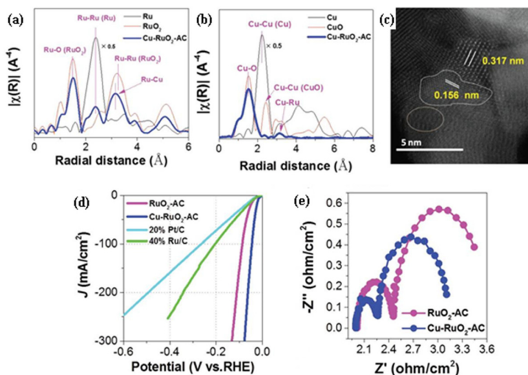
Fig. 1 (a) EXAFS spectrum obtained at the Ru K-edge of Cu–RuO 2 activated in comparison with those of Ru and RuO 2 ; (b) EXAFS spectrum obtained at the Cu K-edge of Cu–RuO 2 activated in comparison with those of Cu and CuO; (c) HAADF-STEM image of Cu–RuO 2 activated , where the oval pink area reveals the obvious lattice distortion; (d) LSV curves for the HER of Cu–RuO 2 activated in comparison with those of RuO 2 –AC, 20% Pt/C and 40% Ru/C; (e) EIS plot for the HER of Cu–RuO 2 activated in comparison with that of RuO 2 –AC obtained at –0.1 V versus RHE (reproduced with permission from ref. 4. Copyright 2023, Wiley-VCH GmbH).
