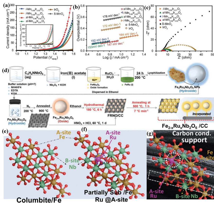
Fig. 5 (a) LSV curves (inset plot depicts LSV curves normalized by ECSA), (b) corresponding Tafel slopes, and (c) Nyquist plots of sl-Mn 0.98 Ir 0.02 O 2 and its counterparts in 0.5 M H 2 SO 4 (reproduced with permission from ref. 1. Copyright 2023, Wiley-VCH GmbH). (d) Schematic diagram depicting the synthesis process for Fe 2-x Ru x Nb 2 O 6 /carbon cloth. Chemical structures of (e) Fe 2 Nb 2 O 6 , (f) Fe 2-x Ru x Nb 2 O 6 , and (g) Fe 2-x Ru x Nb 2 O 6 /carbon cloth depicting the site occupancies in columbite (reproduced with permission from ref. 26. Copyright 2023, Wiley-VCH GmbH).
