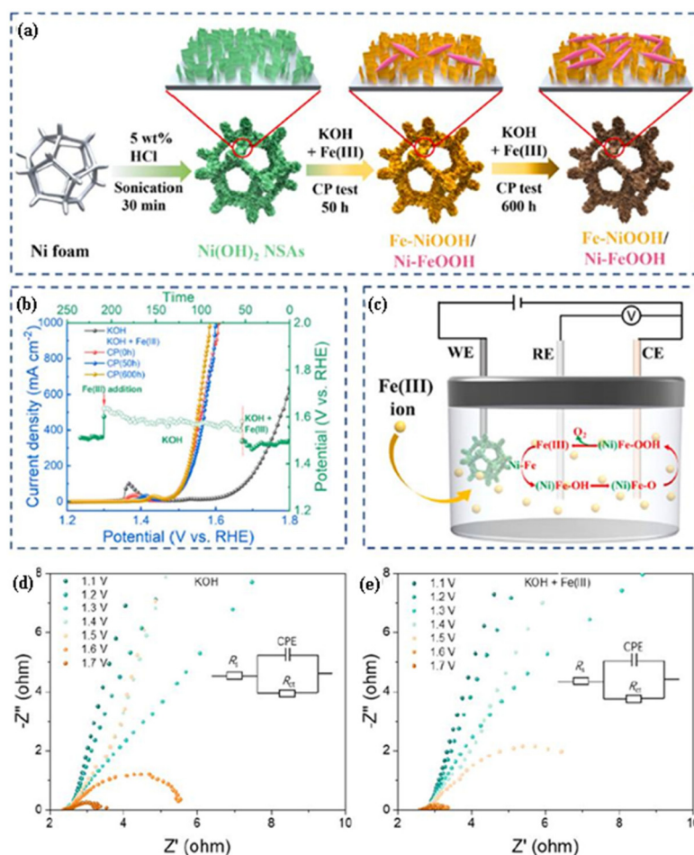
Fig. 2 (a) Schematic diagram representing the synthesis process for \text{Ni}(\text{OH})_2 nanosheet arrays and their subsequent structural evolution during a chronopotentiometry test in 1 M KOH in the presence of 500 \mu\text{M} \text{Fe}(\text{III}) at different time intervals. (b) The LSV and chronopotentiometry plot for the OER of \text{Ni}(\text{OH})_2 in KOH with \text{Fe}(\text{III}) in comparison with those of \text{Ni}(\text{OH})_2 in KOH. (c) Proposed mechanism for the OER on \text{Ni}(\text{OH})_2 in alkaline electrolyte with \text{Fe}(\text{III}) ; CE, RE, and WE are the counter electrode, reference electrode, and working electrode, respectively. Nyquist plot for the OER of (d) \text{Ni}(\text{OH})_2 in KOH with \text{Fe}(\text{III}) in comparison with that of (e) \text{Ni}(\text{OH})_2 in KOH (reproduced with permission from ref. 16. Copyright 2023, Elsevier B.V.).
