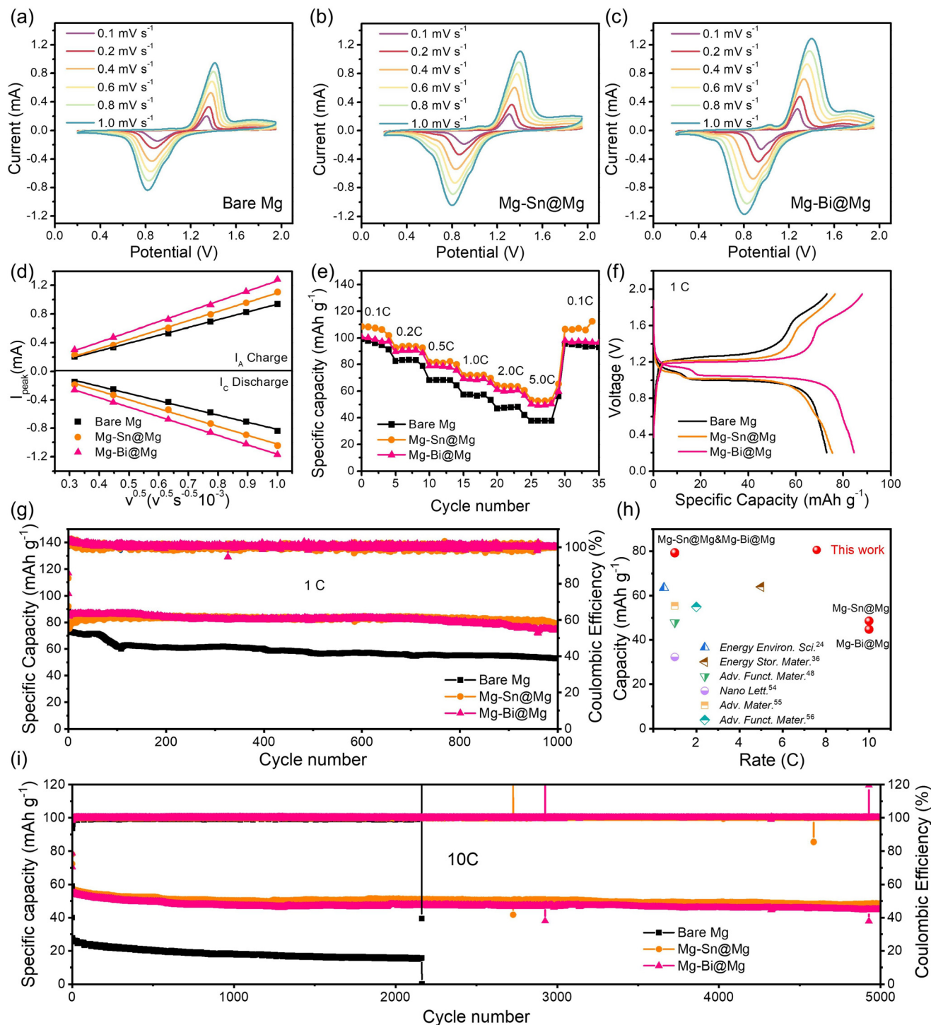
Fig. 6 CV curves of (a) \text{Mo}_6\text{S}_8/\text{bare Mg} , (b) \text{Mo}_6\text{S}_8/\text{Mg-Sn@Mg} and (c) \text{Mo}_6\text{S}_8/\text{Mg-Bi@Mg} full cells at different scan rates from 0.1 to 1.0 \text{mV s}^{-1} in the voltage range of 0.2–1.95 V and (d) the square root of scan rate ( v^{0.5} ) of bare Mg, Mg-Sn@Mg and Mg-Bi@Mg full cells. (e) Rate performance of the \text{Mo}_6\text{S}_8/\text{bare Mg} , \text{Mo}_6\text{S}_8/\text{Mg-Sn@Mg} and \text{Mo}_6\text{S}_8/\text{Mg-Bi@Mg} full cells. (f) The first charge–discharge profiles for \text{Mo}_6\text{S}_8/\text{bare Mg} , \text{Mo}_6\text{S}_8/\text{Mg-Sn@Mg} and \text{Mo}_6\text{S}_8/\text{Mg-Bi@Mg} full cells at 1 C. (g) Cycling performance of the \text{Mo}_6\text{S}_8/\text{bare Mg} , \text{Mo}_6\text{S}_8/\text{Mg-Sn@Mg} and \text{Mo}_6\text{S}_8/\text{Mg-Bi@Mg} full cells at 1 C. (h) The capacity and cycling stability performance of the \text{Mo}_6\text{S}_8/\text{Mg-Sn@Mg} and \text{Mo}_6\text{S}_8/\text{Mg-Bi@Mg} cells compared with those of previously reported \text{Mo}_6\text{S}_8/\text{Mg} full cells. 26,38,55,61–63 (i) Cycling performance of \text{Mo}_6\text{S}_8/\text{bare Mg} , \text{Mo}_6\text{S}_8/\text{Mg-Sn@Mg} and \text{Mo}_6\text{S}_8/\text{Mg-Bi@Mg} full cells at 10 C.
