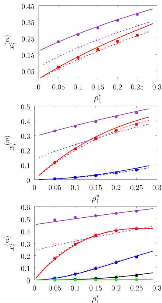
Fig. 6 A fraction of the m times bonded fluid and matrix particles x_i^{(m)} as a function of the fluid density \rho_1^* of the models L1M1 (top panel), L1M2 (intermediate panel), and L1M4 (bottom panel) at different values of \eta_0 , i.e. \eta_0 = 0.1 (dashed lines and open circles) and \eta_0 = 0.2 (solid lines and filled circles). Here a fraction of the singly bonded fluid particles ( m = 1 ) are shown by the violet lines and symbols and for the matrix particles we have: m = 1 (red curves and symbols), m = 2 (blue lines and symbols), m = 3 (black lines and symbols), and m = 4 (green line and symbols). The theoretical results are represented by the lines and the computer simulation results are represented by the symbols.
