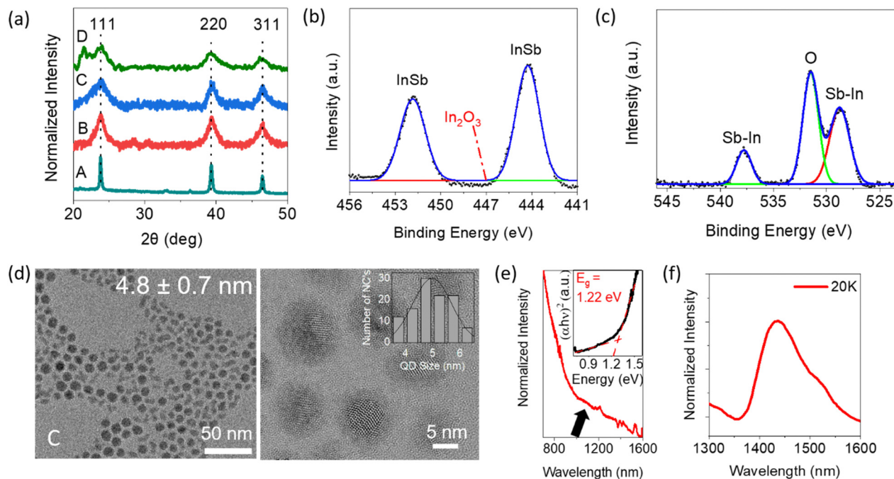
Fig. 1 (a) Powder XRD patterns of the products prepared with different centrifugation processes; a detailed scheme has been added in Scheme S1 (see ESI†). XPS spectra in (b) In 3d and (c) Sb 3d core levels of sample C, fitted with a Gaussian function. (d) HR-TEM image of sample C with the size distribution profile shown in the inset. (e) Room-temperature NIR absorption spectrum of sample C dispersed in TCE. (f) PL spectra of sample C at a temperature of 20 K.
