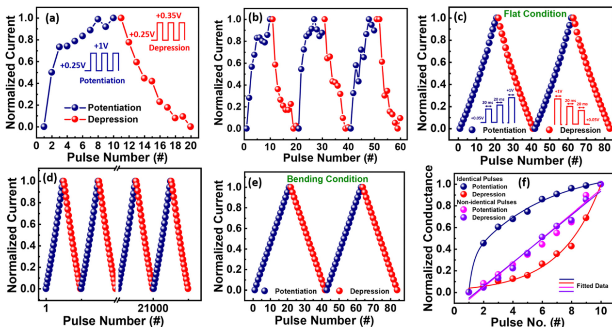
Fig. 5 (a) Single P&D cycle by giving identical pulses of 1 V with constant read voltage of 0.25 V. (b) Multiple cycles of P&D via identical pulses pattern. (c) and (d) are P&D obtained by non-identical pulse method in flat condition. (e) P&D cycles in bending condition obtained by non-identical pulse method. (f) Non-linearity factor calculated for P&D obtained by identical pulse and non-identical pulse method.
