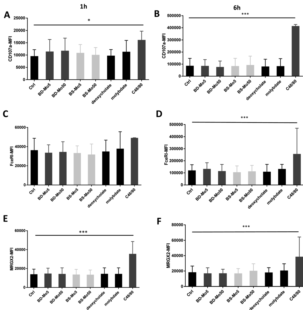
Fig. 2 MoS 2 did not have detrimental impact on mast cell activation markers. CD107a expression of mast cells treated with 5, 50 \mu\text{g mL}^{-1} BD- or BS-MoS 2 for (A) 1 h (B) 6 h. FcεRI expression of mast cells treated with 5, 50 \mu\text{g mL}^{-1} BD- or BS-MoS 2 for (C) 1 h (D) 6 h. MRGX2 expression of mast cells treated with 5, 50 \mu\text{g mL}^{-1} BD- or BS-MoS 2 for (E) 1 h (F) 6 h. All experiments were conducted thrice in triplicate and shown as mean \pm SD. * P < 0.05 ; ** P < 0.01 , *** P < 0.001 by one-way ANOVA with Bonferroni post-tests.
