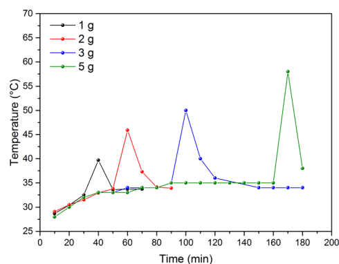
Fig. 8 External bowl temperature as a function of milling time with varying powder mass. Milling conditions: 450 rpm, 7 \times 10 mm balls, no rest time, and n_{Al}/n_{Co} = 1.0 .
