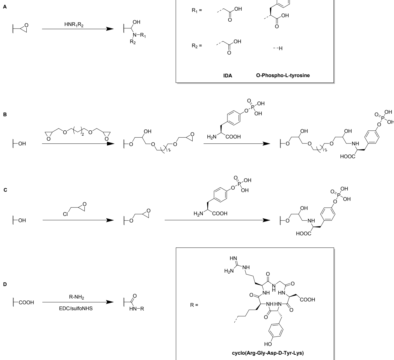
Figure 35 Schematic representation of the subsequent modification of hybrid cryogels by the direct functionalization of epoxide groups with amines such as IDA or o-phospho-L-tyrosine (A), or via the modification of hydroxy groups by the introduction of epoxy groups using 1,4-butanedioldiglycidyl ether (B) or epichlorohydrin (C). Alternative strategies include the attachment of peptides such as cyclo(Arg-Gly-Asp-D-Tyr-Lys) via EDC/sulfoNHS coupling towards cryogel carboxylic acid groups (D).
