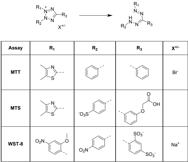
Figure 10 Schematic representation of the underlying chemical reactions of the colorimetric assays which utilize the reduction of tetrazolium dyes such as 3-(4,5-dimethylthiazol-2-yl)-2,5-diphenyltetrazolium bromide (MTT), (3-(4,5-dimethylthiazol-2-yl)-5-(3-carboxymethoxyphenyl)-2-(4-sulfophenyl)-2H-tetrazolium) (MTS) or (2-(2-methoxy-4-nitrophenyl)-3-(4-nitrophenyl)-5-(2,4-disulfophenyl)-2H-tetrazolium) (WST-8) to the corresponding formazan.
