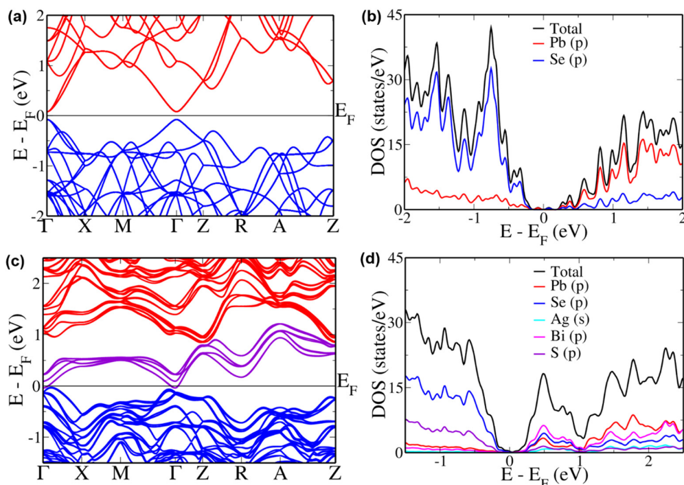
Fig. 5 Electronic structures and pDOS of (a) and (b) PbSe and (c) and (d) \text{AgBiSeS} alloyed PbSe. Energies are shifted with respect to Fermi level, which is set to zero.
