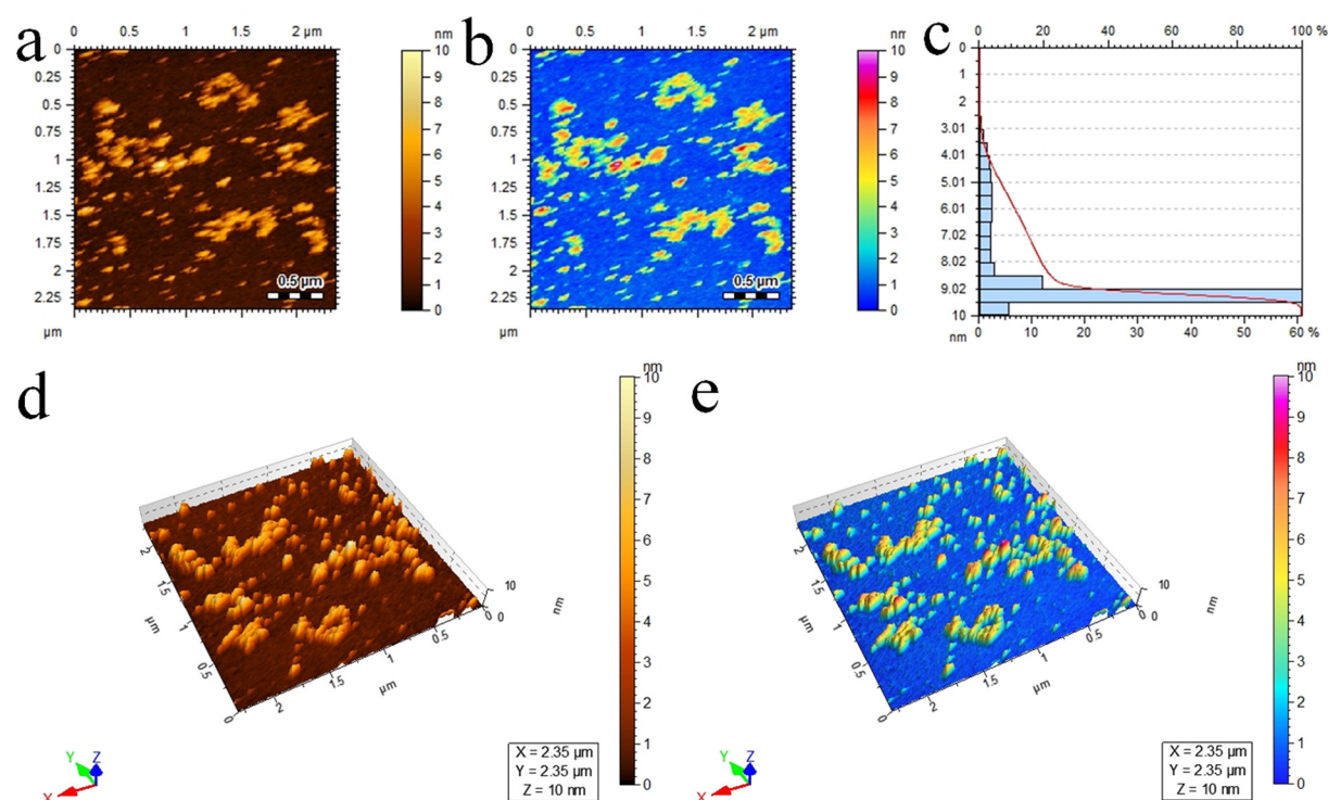
Fig. 5 AFM results of \text{Pd@Ti}_3\text{C}_2\text{T}_x\text{-TiO}_2 photocatalysts: (a) and (b) 2D-tapping modes, (c) size distribution and (d) and (e) 3D images.
