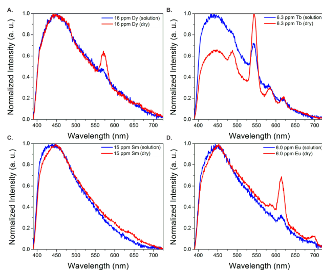
Fig. 3 Normalized emission spectra of BTC-1 with Dy (A), Tb (B), Sm (C), and Eu (D) in solution and after drying. Drying significantly enhances the emission signal from the REEs.
