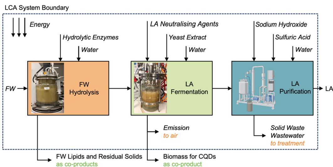
Fig. 1 System boundary diagram. Italics indicate the connection to background LCI databases. FW: food waste. LA: lactic acid. LA neutralising agents: NaOH, shell, Ca(OH) 2 . Glucoamylase is used in FW hydrolysis in the simulation process.
