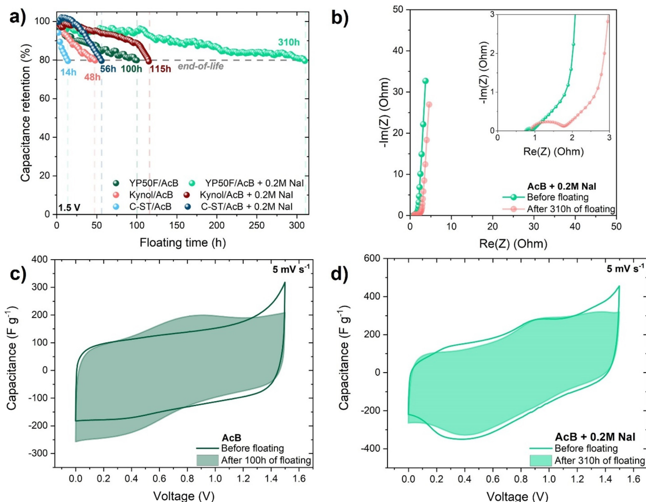
Fig. 4 (a) Capacitance retention of different microporous carbons (YP50F, Kynol, and C-ST) based ECs operating in acetate buffer with and without 0.2 mol \text{L}^{-1} NaI additive during the floating test (at 1.5 V). (b) Nyquist plots obtained from YP50F-based ECs operating in acetate buffer + 0.2 mol \text{L}^{-1} NaI before and after 310 h floating test. Cyclic voltammogram at 5 \text{ mV s}^{-1} recorded for (c) acetate buffer before and after 100 h floating test; (d) acetate buffer + 0.2 mol \text{L}^{-1} NaI before and after 310 h floating test.
