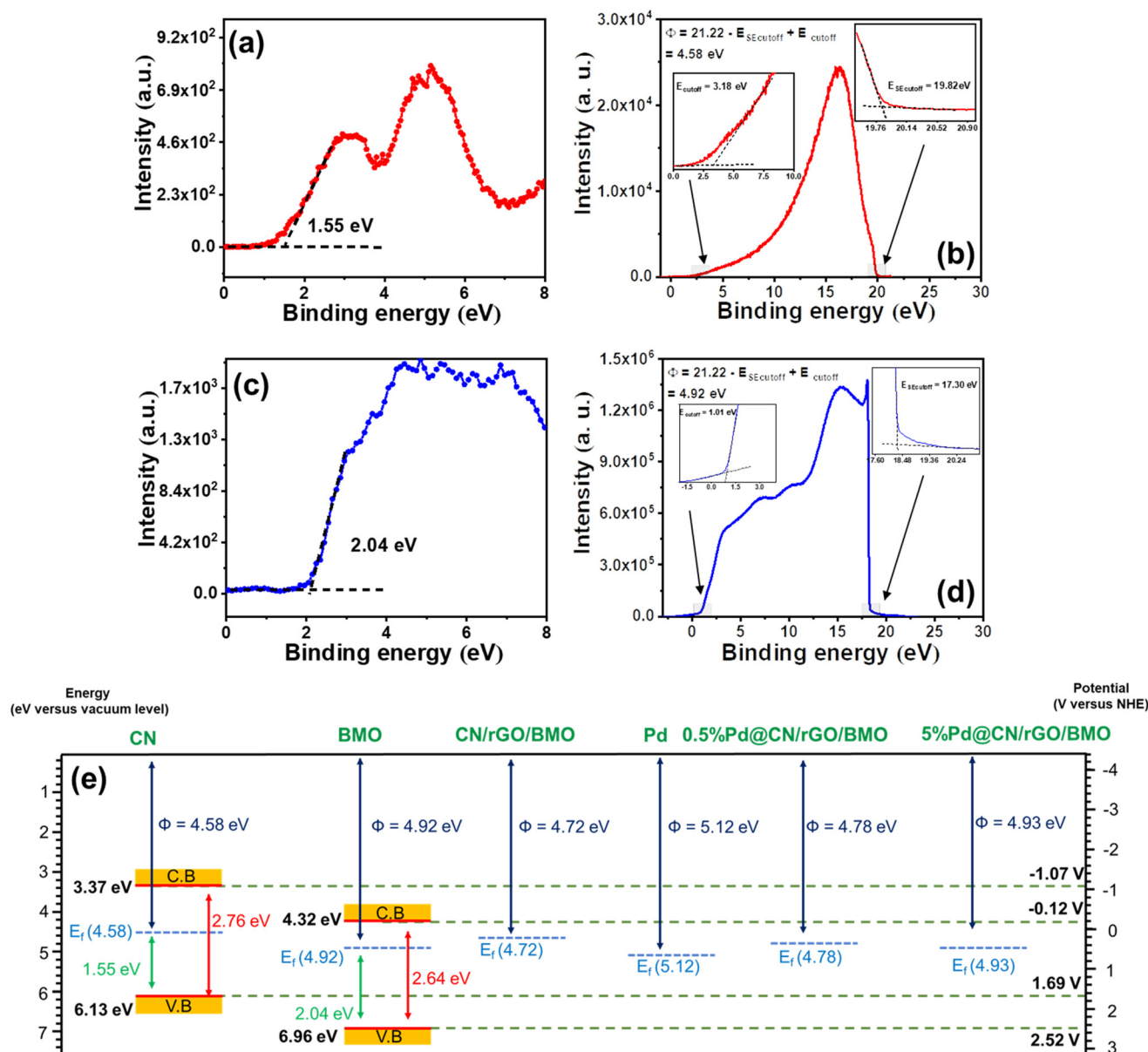
Fig. 6 (a) VB-XPS spectrum for CN, (b) UPS spectrum for CN, (c) VB-XPS spectrum for BMO, and (d) UPS spectrum for BMO and (e) (a)calculated band-structures for CN, BMO, CN/rGO/BMO(2 : 1), 0.5%Pd@CN/rGO/BMO(2 : 1), and 5%Pd@CN/rGO/BMO(2 : 1).
