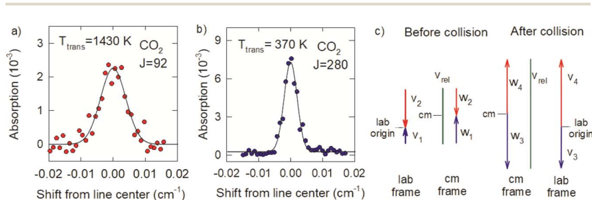
Fig. 11 Doppler-broadened line profiles for \text{CO}_2 (a) J = 92 and (b) J = 280 at 200 ns following the optical centrifuge pulse. (c) Velocity vectors in the lab frame ( v ) and center of mass (cm) frame ( w ) for a collision with b = 0 of an optically centrifuged molecule and a thermal bath molecule, before (1, 2) and after (3, 4) collisional energy transfer.
