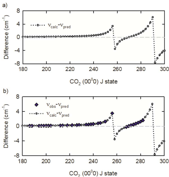
Fig. 4 (a) A comparison of calculated ( v_{\text{calc}} ) and predicted ( v_{\text{pred}} ) transition frequencies for \text{CO}_2 R-branch transitions. (b) A comparison of observed transition frequencies v_{\text{obs}} with the calculated and predicted values.
