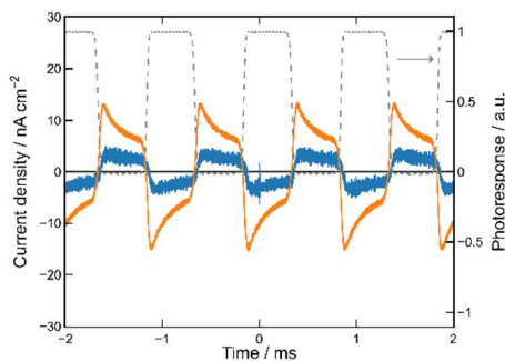
Fig. 4 Time trajectory of the transient photocurrent for the [ITO||S||Ag] photocell. The orange and blue curves show the photocurrent when S = \text{ET-PRBT} and \text{EO-PRBT} , respectively, and the gray broken curve indicates the response from a Si diode to monitor the light-on and -off periods.
