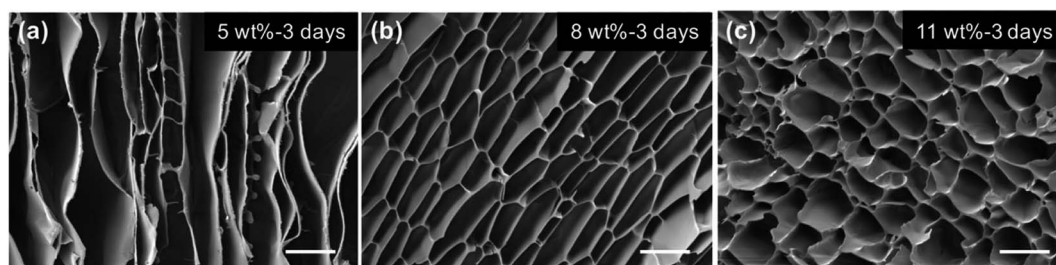
Fig. 7 SEM images of porous starch with starch concentrations of 5 wt% (a), 8 wt% (b) and 11 wt% (c). Scale bars are 20 μm. 119
